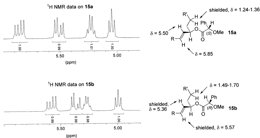
Figure 5. Assignment of the relative configuration at the stereogenic center C-5.
