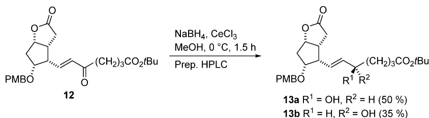
Scheme 6. Preparation of the diastereomeric alcohols 13a and 13b .
