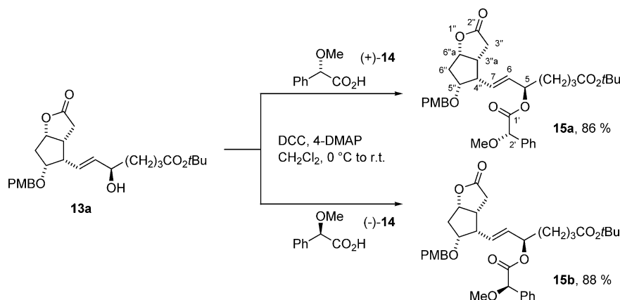
Scheme 7. Esterification of alcohol 13a with (S) - and (R) -O-methylmandelic acid.
