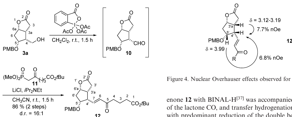
Scheme 5. Preparation of enone 12 .
