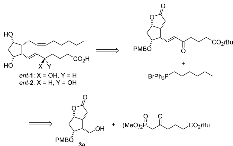
Scheme 4. General strategy for the syntheses of isoprostanes ent-1 and ent-2 .
