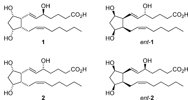
Figure 2. Stereoisomeric isoprostanes of the 5-F 2 -IsoP series.
