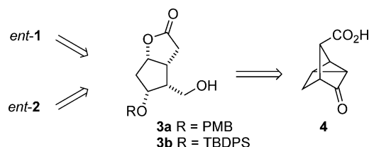
Scheme 1. Lactones of type 3 as key intermediates for syntheses of isoprostanes.
