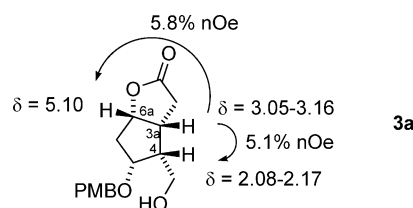
Figure 3. Nuclear Overhauser effects observed for lactone 3a .
