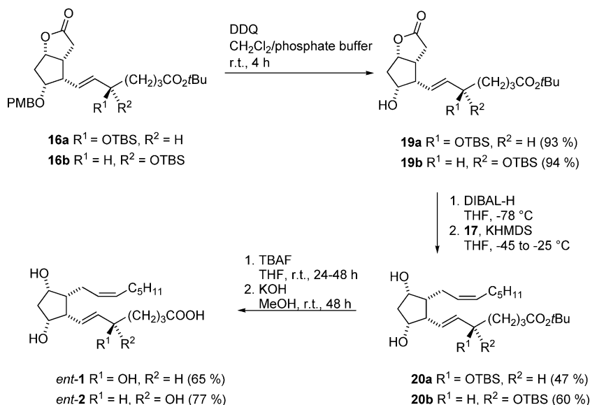
Scheme 9. Completion of the synthesis of isoprostanes ent-1 and ent-2 .
