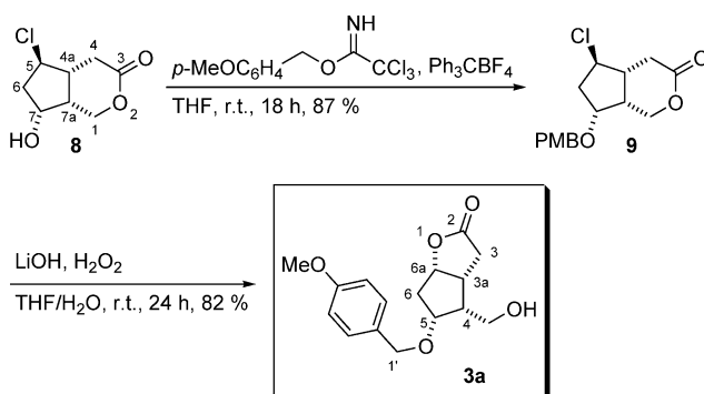
Scheme 3. Synthesis of key intermediate 3a .
