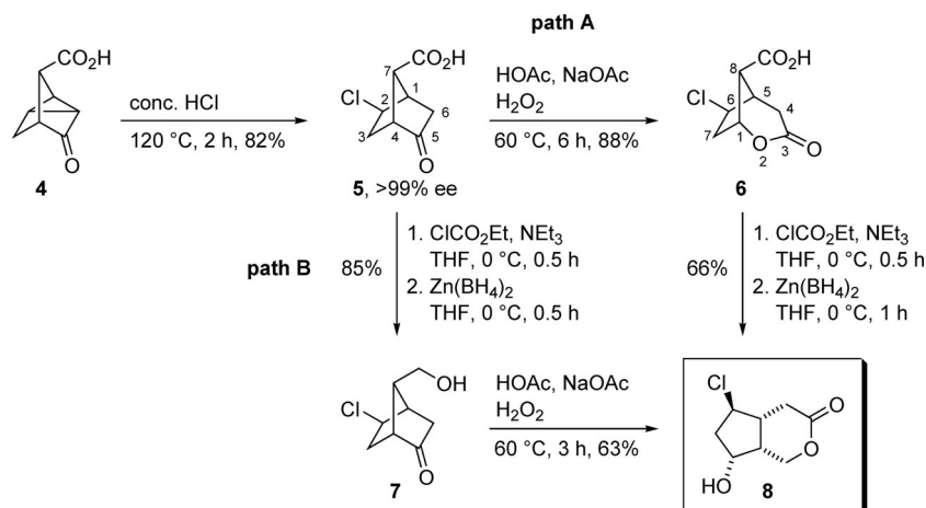
Scheme 2. Synthesis of the bicyclic lactone 8 .
