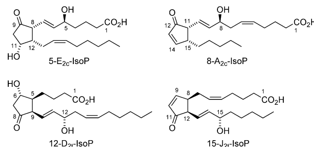
Figure 1. Important classes of isoprostanes.
