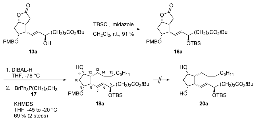
Scheme 8. First attempt to synthesize compounds 20 .
